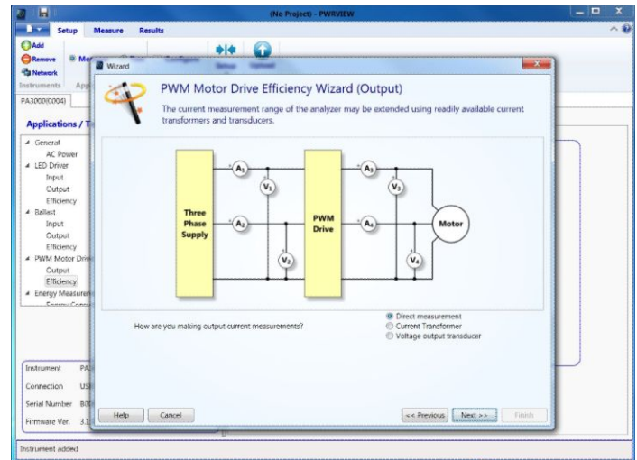
PWM Motor Efficiency Wizard in the PWRVIEW software
